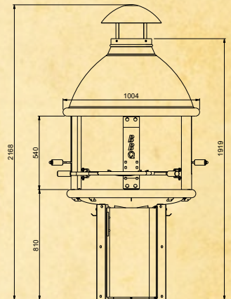
TUNDRA GRILL® BBQ HIGH MODEL
