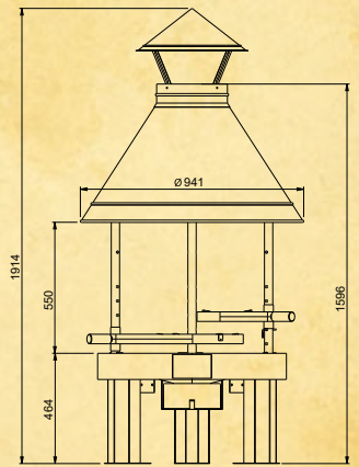
TUNDRA GRILL® 80 LOW MODEL
