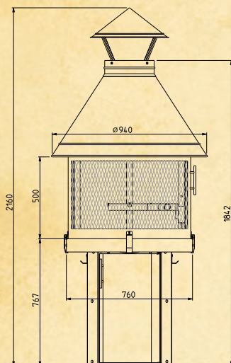
TUNDRA GRILL® CITY HIGH MODEL
