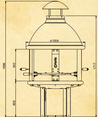
TUNDRA GRILL® BBQ LOW MODEL
