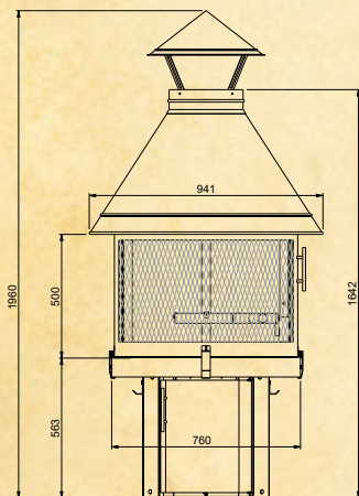
TUNDRA GRILL® CITY LOW MODEL
