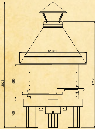
TUNDRA GRILL® 100 LOW MODEL
