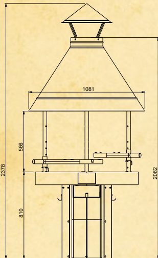
TUNDRA GRILL® 100 HIGH MODEL
