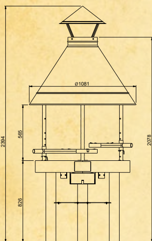
TUNDRA GRILL® HEAVY DUTY HIGH MODEL
