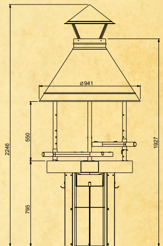
TUNDRA GRILL® 80 HIGH MODEL
